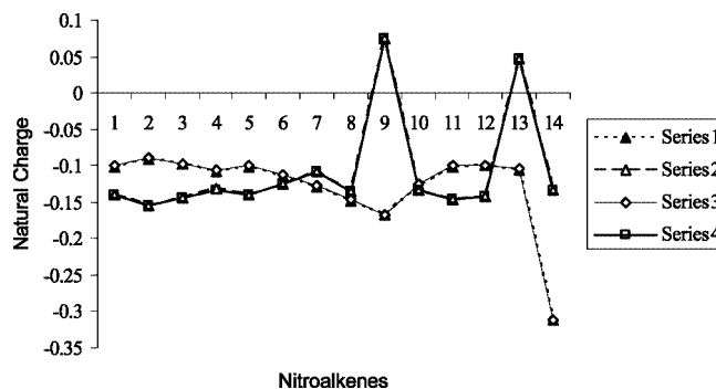
Figure 3. Distribution of charge at the \beta - and \alpha -C atoms in nitroalkenes 1–14 . Series 1 and 2: electron density at the \beta - and \alpha -C atoms, respectively, with Method B: MP2/6-31G(d)//B3LYP/6-31G(d); Series 3 and 4: electron density at the \beta - and \alpha -C atoms, respectively, with Method C: MP2/6-31G(d)//B3LYP/6-31+G(d); overlapping of Series 1 & 3 and Series 2 & 4 shows the reliability of the \beta -CED and \alpha -CED as calculated by the applied methods.
