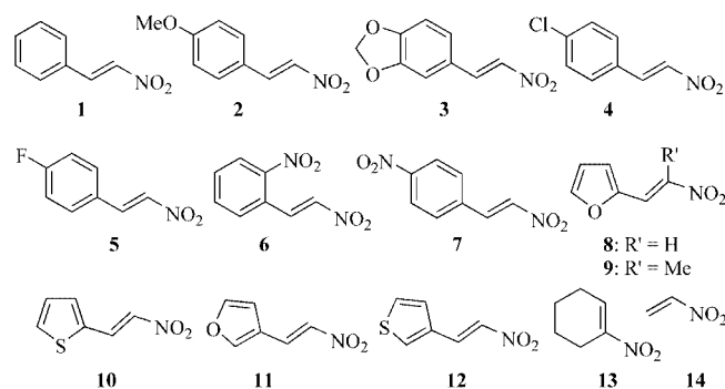
Figure 1. Nitroalkenes chosen for evaluation of reactivity in conjugate additions.
