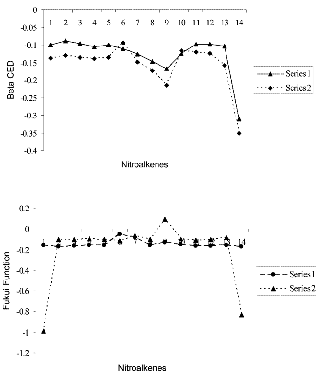
Figure 4. Comparison of the trends of the \beta -CED and f_{\beta-C}^{+} derived by natural and Mulliken charges. Series 1: natural charge derived \beta -CED and f_{\beta-C}^{+} , respectively; Series 2: MPA derived \beta -CED and f_{\beta-C}^{+} , respectively.
