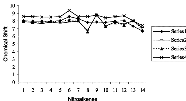
Figure 2. Correlation of theoretical and experimental chemical shift values for the proton \beta and cis to the \text{NO}_2 group in nitroalkenes 1–14 ; Series 1: exp. \delta ; Series 2: calcd. \delta (Method A); Series 3: calcd. \delta (Method B); Series 4: calcd. \delta (Method C).
